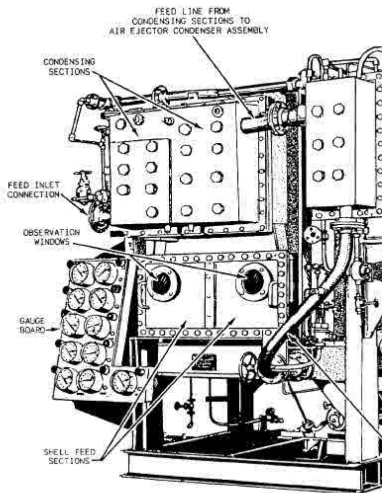
Figure 10-32.—Two-stage flash-type
